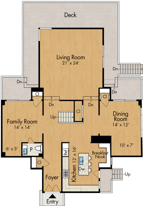
Main Level 1,765 SQ FT
